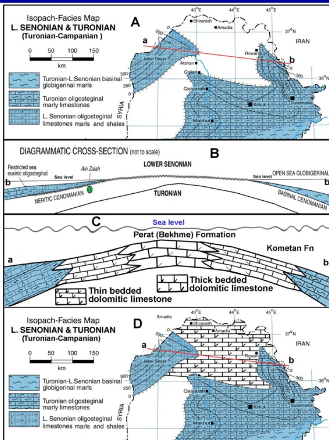
Fig. (7) A and B) Facies maps of Cretaceous and related geologic cross section along the red line (ab) (Dunnington, 1958 and Aqrav, et al. 2010 ) which shows studied area (white area). C and D) modification of the section and facies map to agree with the result of the present study.
